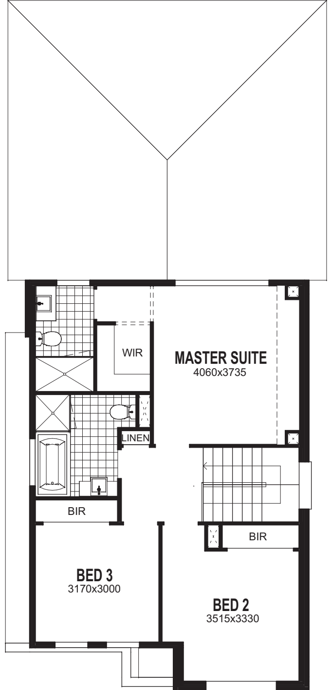
First Floor
